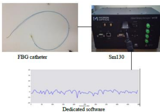
Figure 2 experimental device
